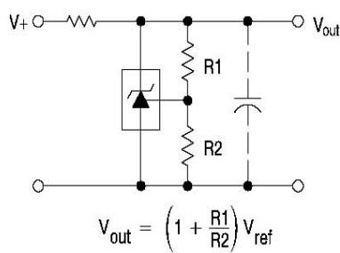
Shutdown Regulator
