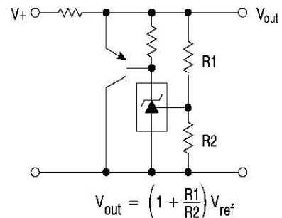
Higher-current Shunt
