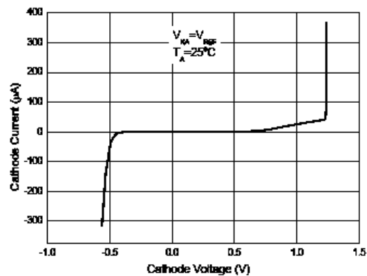
Figure 10. Current vs. cathode Voltage
