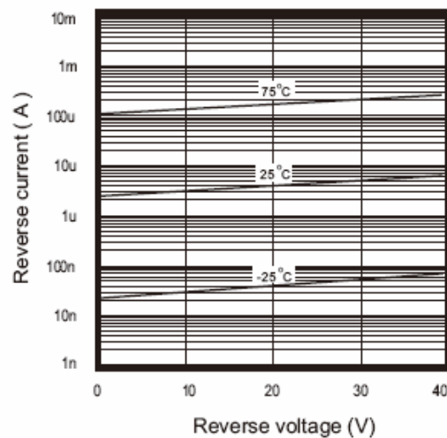
Fig. 2 - Reverse characteristics
