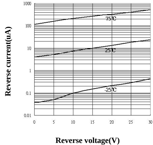
Fig.2-Reverse characteristics
