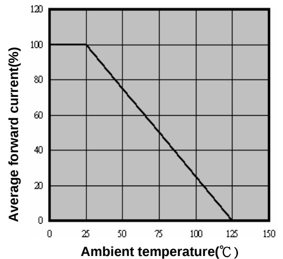
Fig.4-Current derating curve
